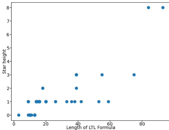
Fig. 12: Visualization complexity metrics for formulas collected from Acacia [16] and NASA’s AAC [24].
